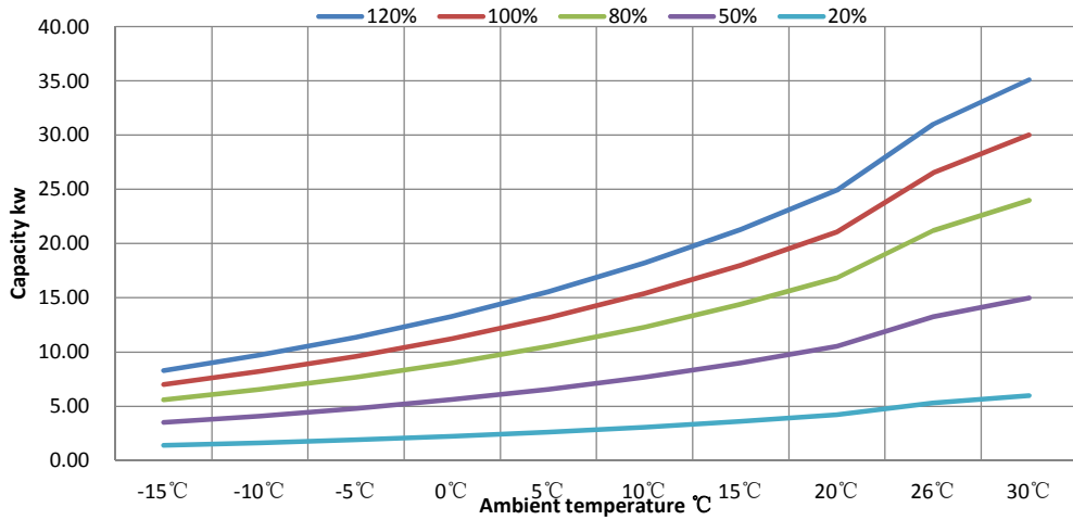
AXCR28T COP Curve
