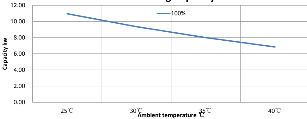
AXCR17 Cooling Capacity Curve
