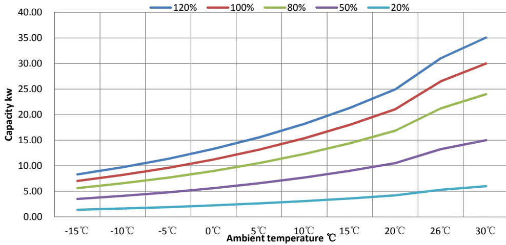
AXCR28 COP Curve
