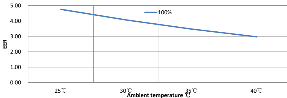
AXCR17 EER Curve
