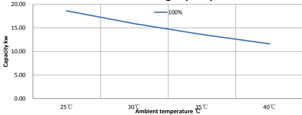
AXCR28T Cooling Capacity Curve
