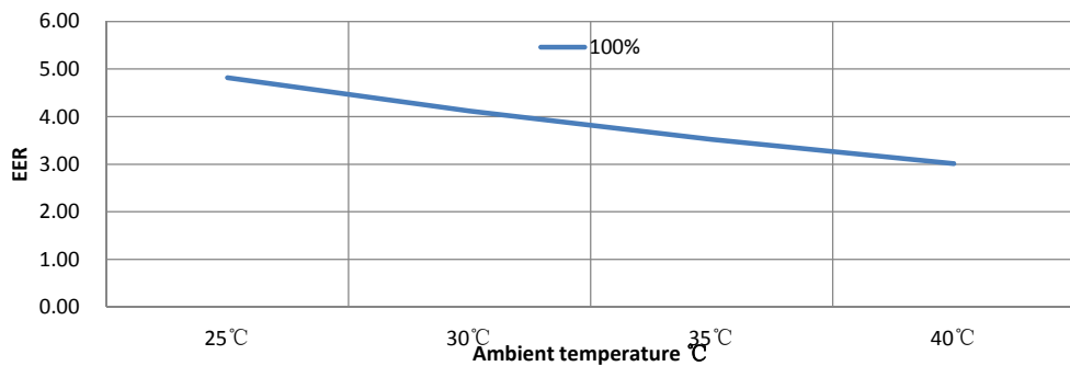
AXCR28T EER Curve
