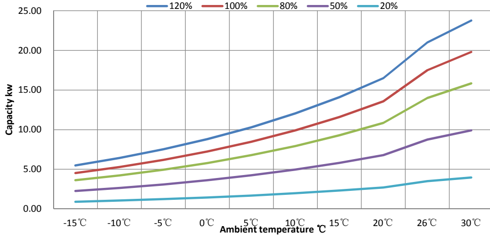
AXCR17 COP Curve
