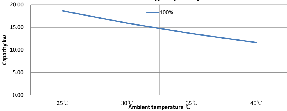
AXCR28 Cooling Capacity Curve
